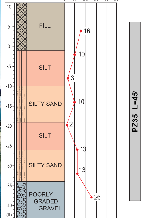
Borehole Data 0 10 20 30 40 50
