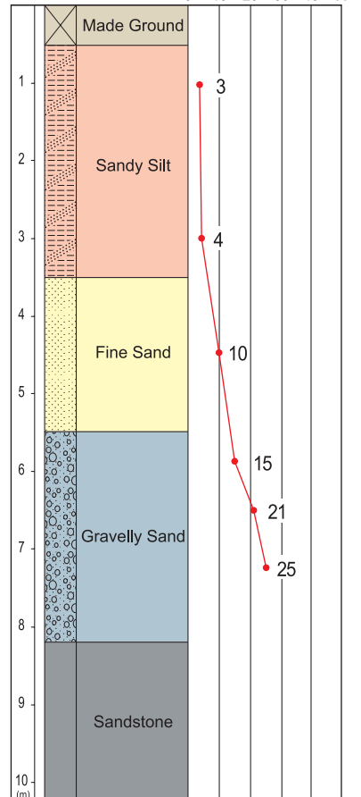
Borehole Data SPT Value
