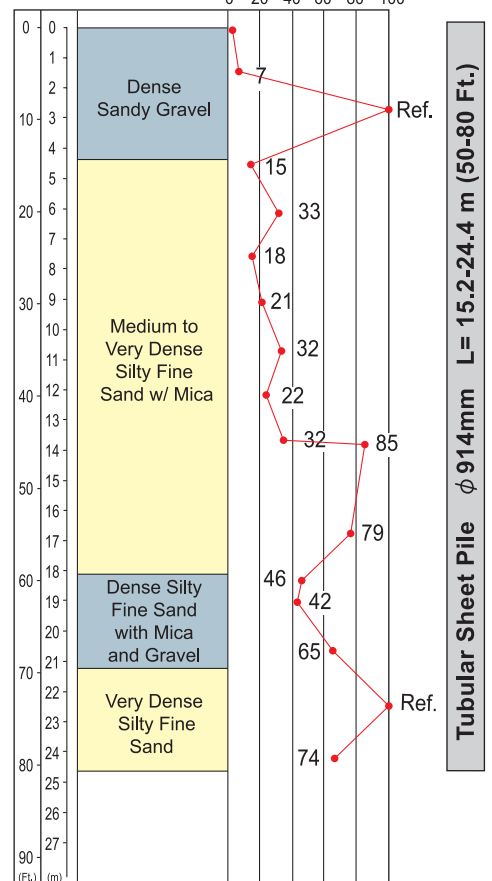
Borehole Data
