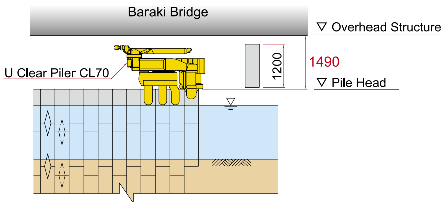
▼ Cross-section
