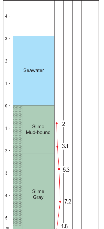
Borehole Data (Pressuremeter) E m (MPa)
