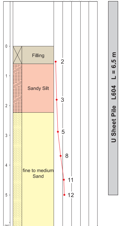
Borehole Data 0 10 20 30 40 50 SPT Value
